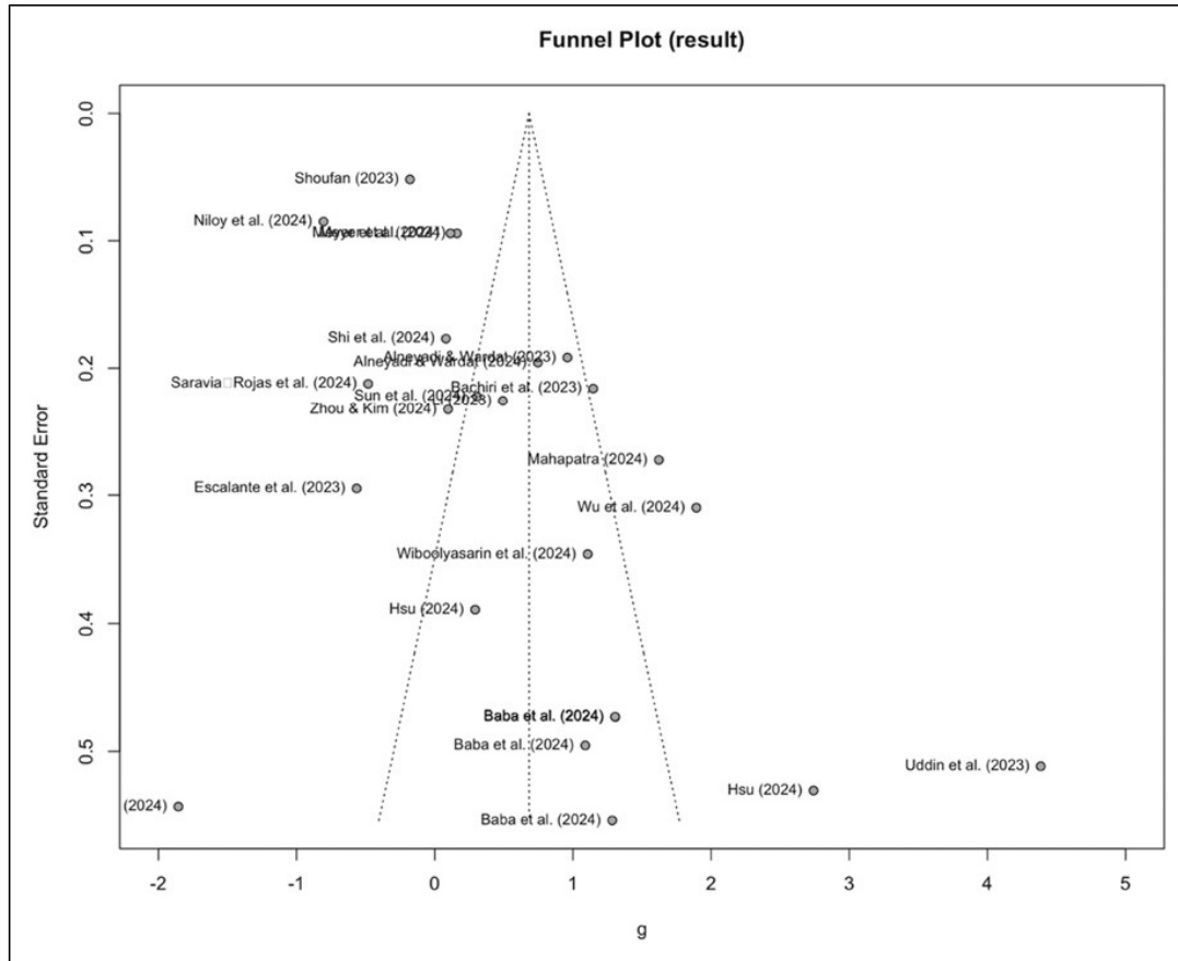
Figure 4. Funnel Plot.
