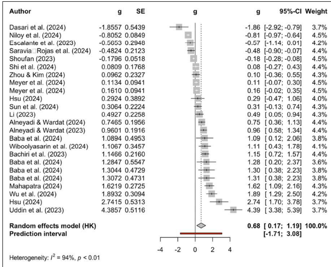
Figure 2. Forest Plots of Effect Sizes.
