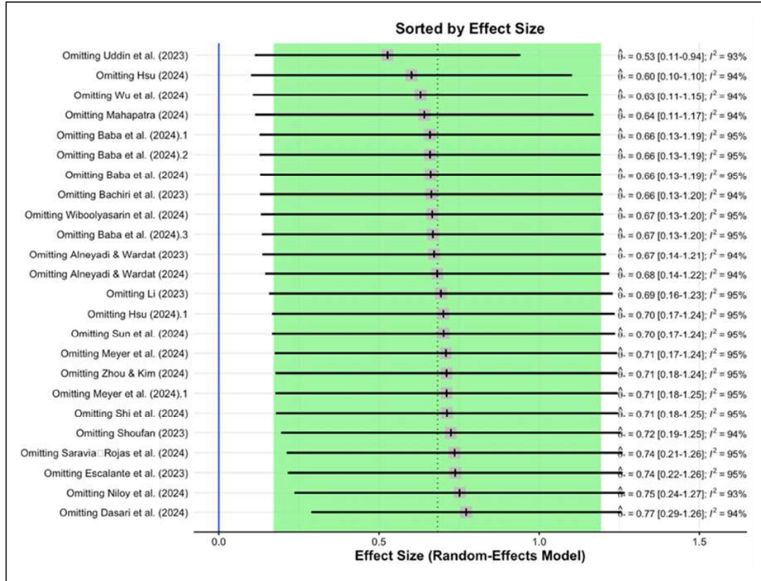
Figure 3. Sensitivity Analysis Leaving Out Each Study.
